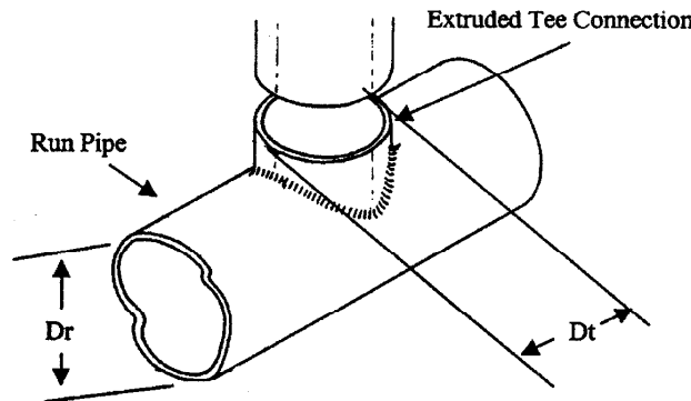
FIG. 1 Extruded Tee Connection
